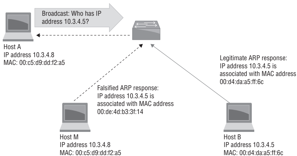
FIGURE 7.4 ARP spoofing
