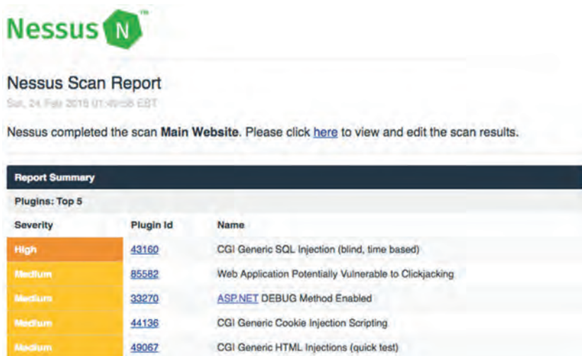
FIGURE 4.4 Sample Nessus scan report
